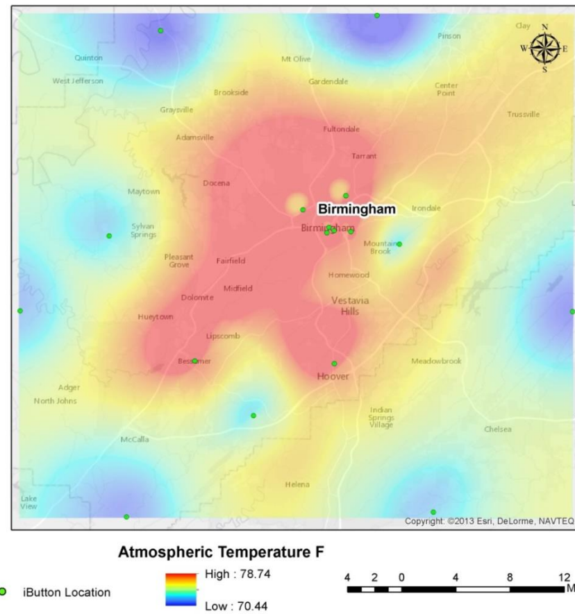
Figure 28. Average atmospheric nighttime temperature for August 2014 in Birmingham.
