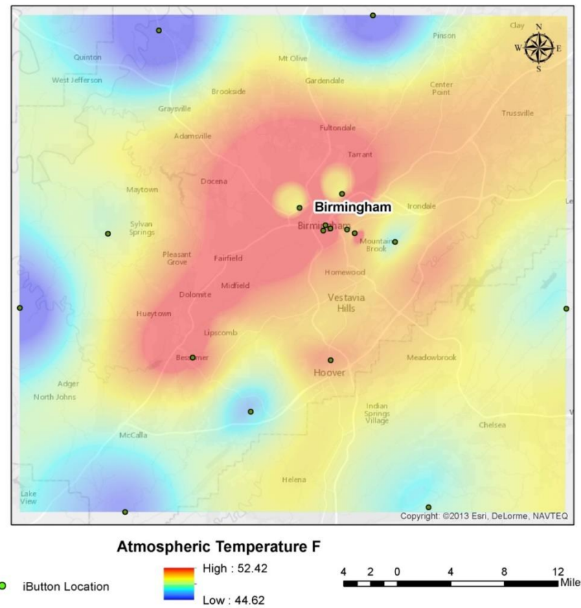
Figure 8. Average atmospheric nighttime temperature for March 2014 in Birmingham.
