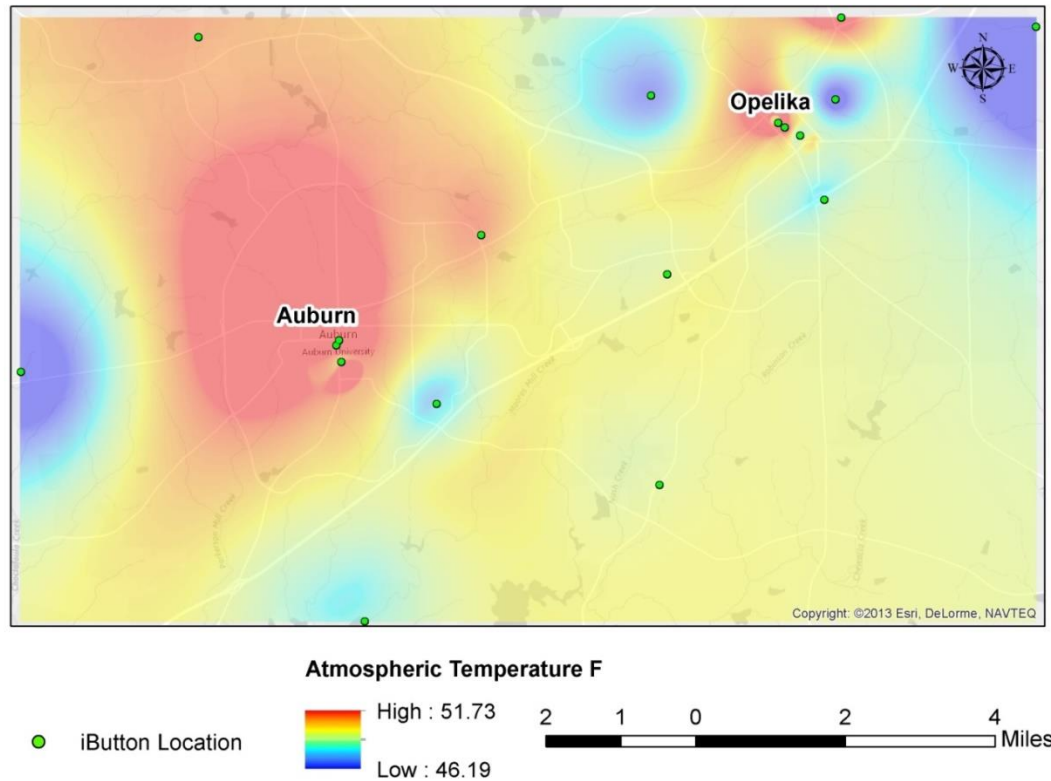
Figure 10. Average atmospheric nighttime temperature for March 2014 in Auburn-Opelika.
