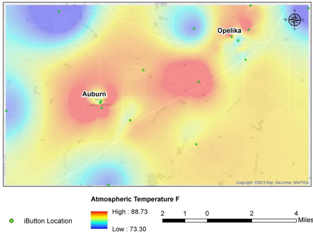
Figure 17. Average atmospheric daytime temperature for May 2014 in Auburn-Opelika.
