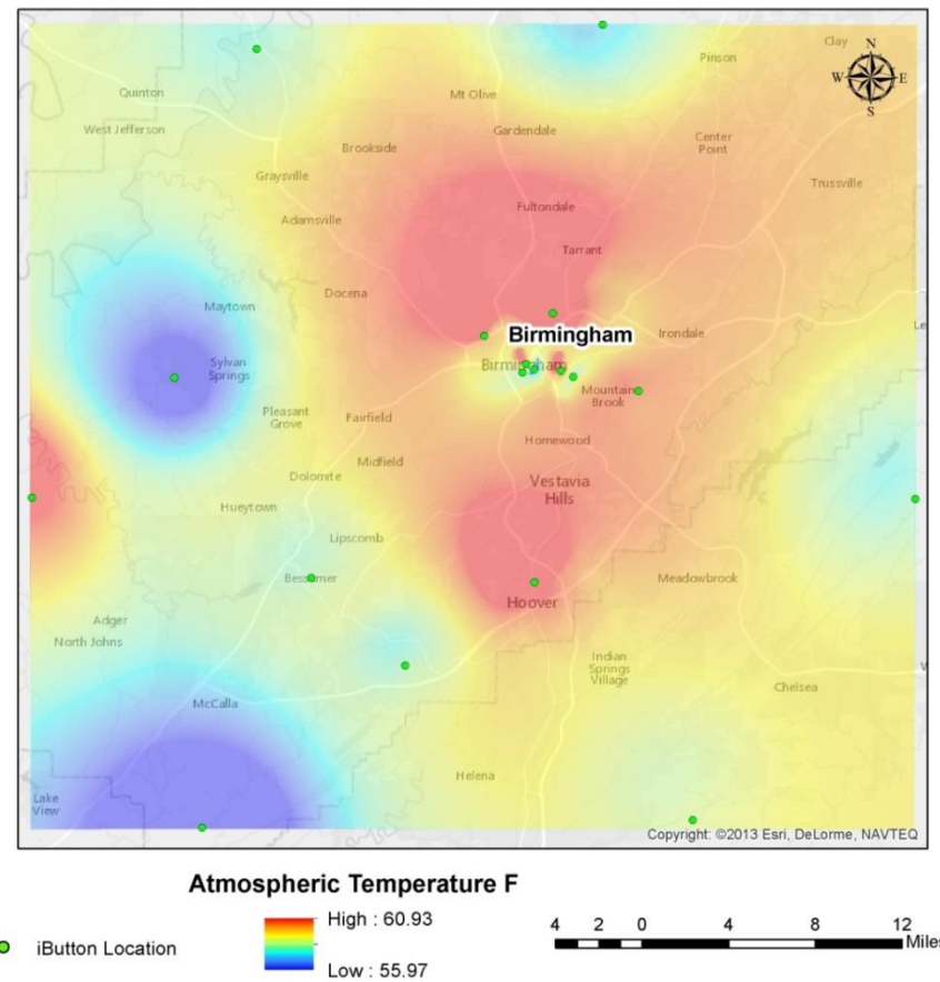
Figure 7. Average atmospheric daytime temperature for March 2014 in Birmingham
