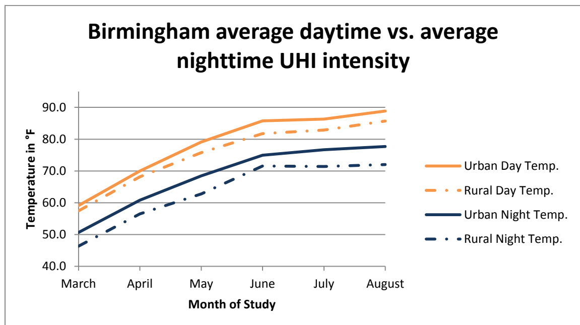
Figure 31. Average urban and rural temperatures for Birmingham.
