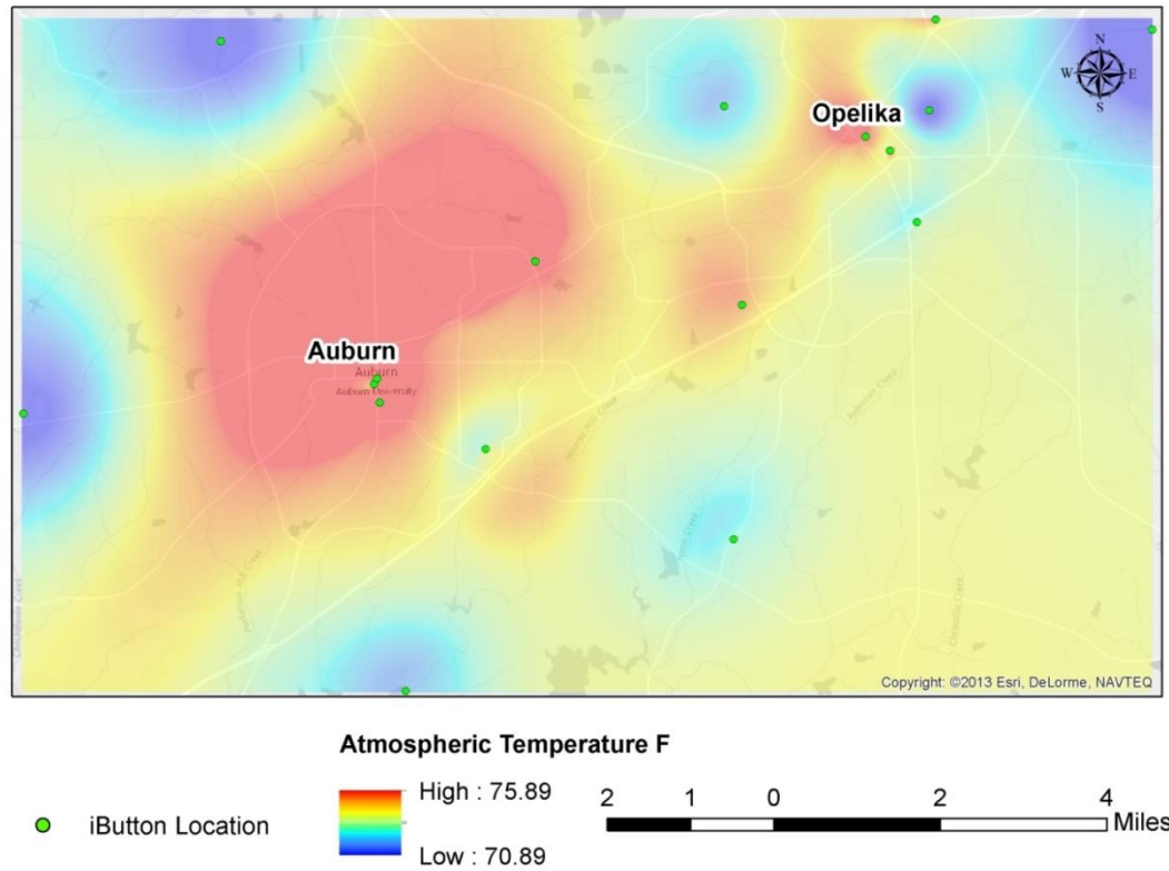
Figure 22. Average atmospheric nighttime temperature for June 2014 in Auburn-Opelika.
