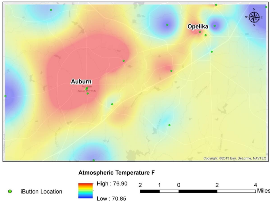
Figure 30. Average atmospheric nighttime temperature for August 2014 in Auburn-Opelika.
