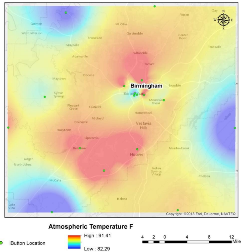
Figure 27. Average atmospheric daytime temperature for August 2014 in Birmingham.
