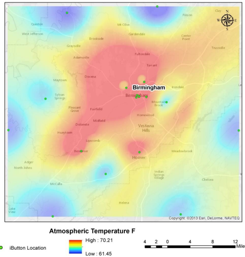
Figure 16. Average atmospheric nighttime temperature for May 2014 in Birmingham.
