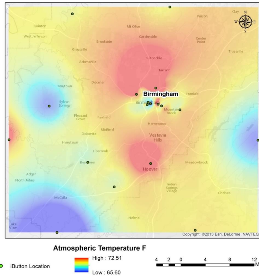
Figure 11. Average atmospheric daytime temperature for April 2014 in Birmingham.
