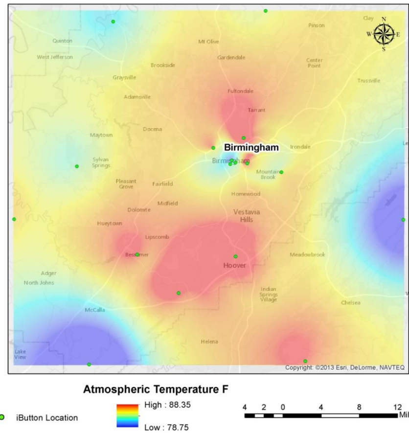
Figure 23. Average atmospheric daytime temperature for July 2014 in Birmingham.
