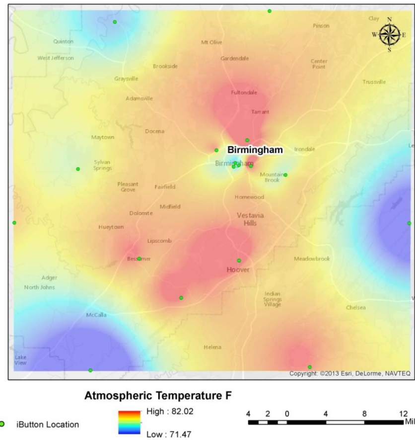
Figure 15. Average atmospheric daytime temperature for May 2014 in Birmingham.
