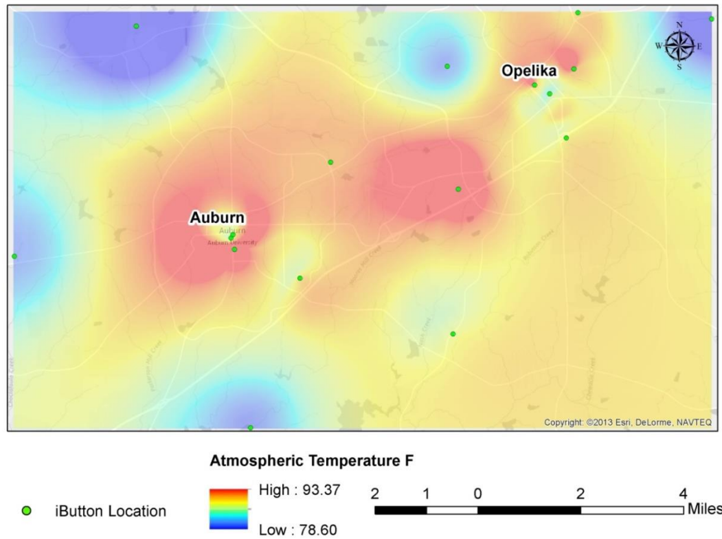
Figure 25. Average atmospheric daytime temperature for July 2014 in Auburn-Opelika.
