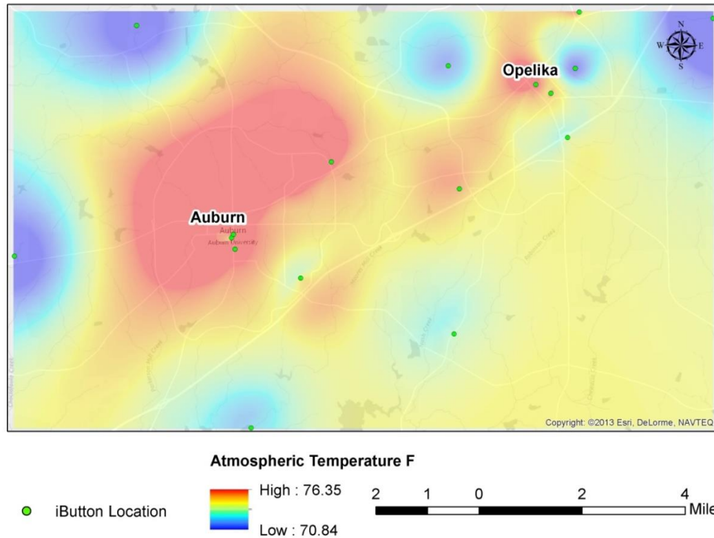
Figure 26. Average atmospheric nighttime temperature for July 2014 in Auburn-Opelika.
