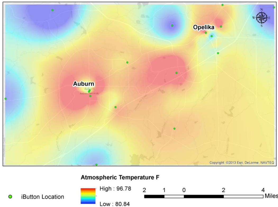
Figure 29 Average atmospheric daytime temperature for August 2014 in Auburn-Opelika.
