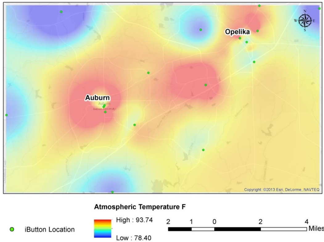
Figure 21. Average atmospheric daytime temperature for June 2014 in Auburn-Opelika.
