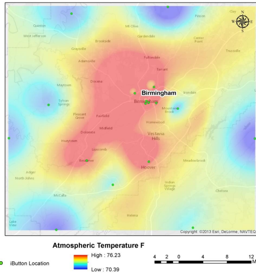
Figure 20. Average atmospheric nighttime temperature for June 2014 in Birmingham.
