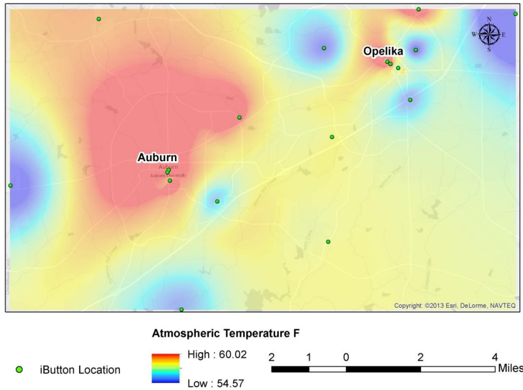
Figure 14. Average atmospheric nighttime temperature for April 2014 in Auburn-Opelika.
