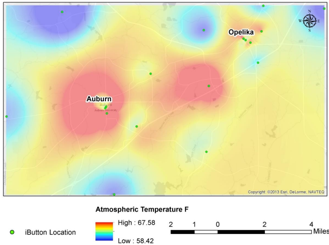
Figure 9. Average atmospheric daytime temperature for March 2014 in Auburn-Opelika.
