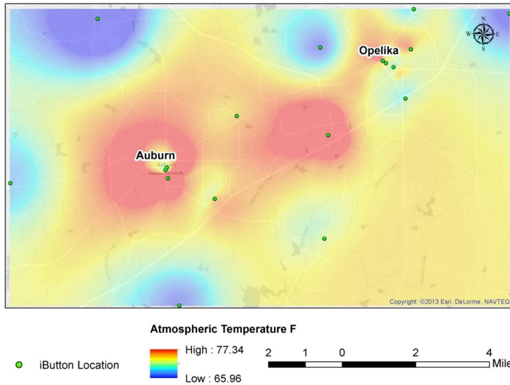
Figure 13. Average atmospheric daytime temperature for April 2014 in Auburn-Opelika.
