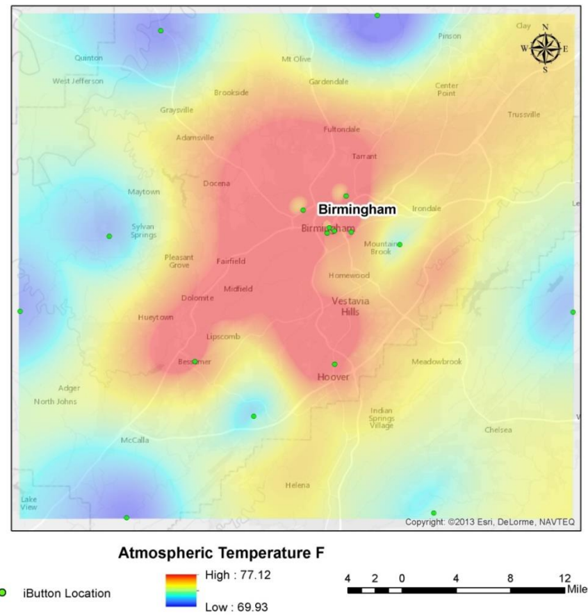
Figure 24. Average atmospheric nighttime temperature for July 2014 in Birmingham.
