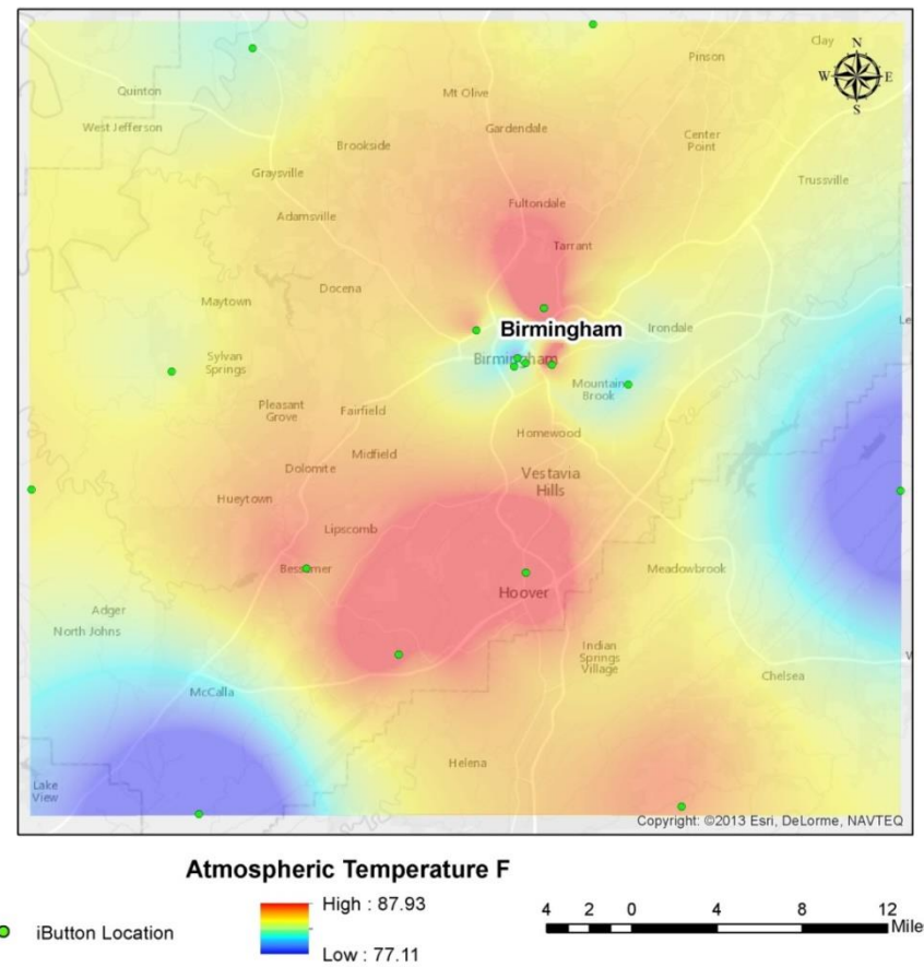
Figure 19. Average atmospheric daytime temperature for June 2014 in Birmingham.
