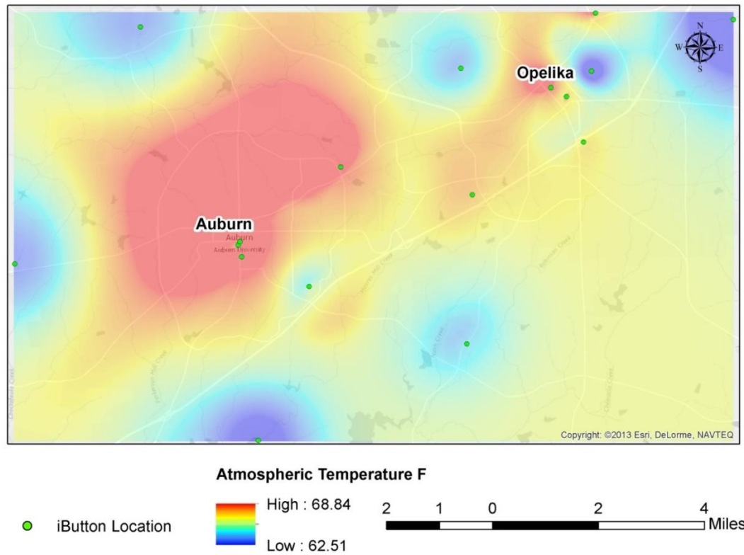
Figure 18. Average atmospheric nighttime temperature for May 2014 in Auburn-Opelika.
