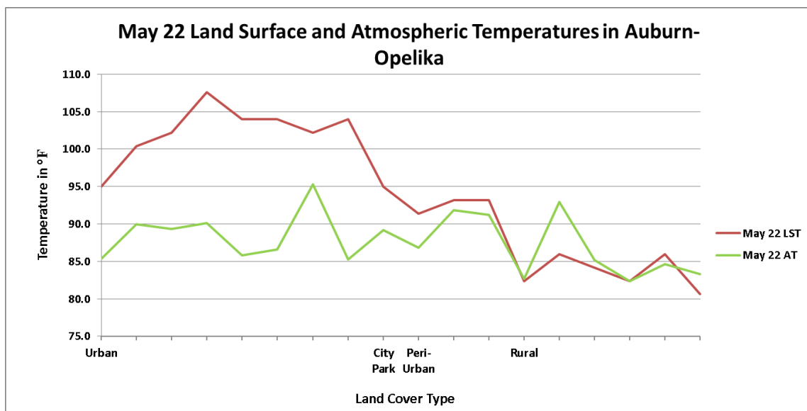
Figure 41 LST and atmospheric temperature change over land cover on 22 May 2014 in Auburn-Opelika
